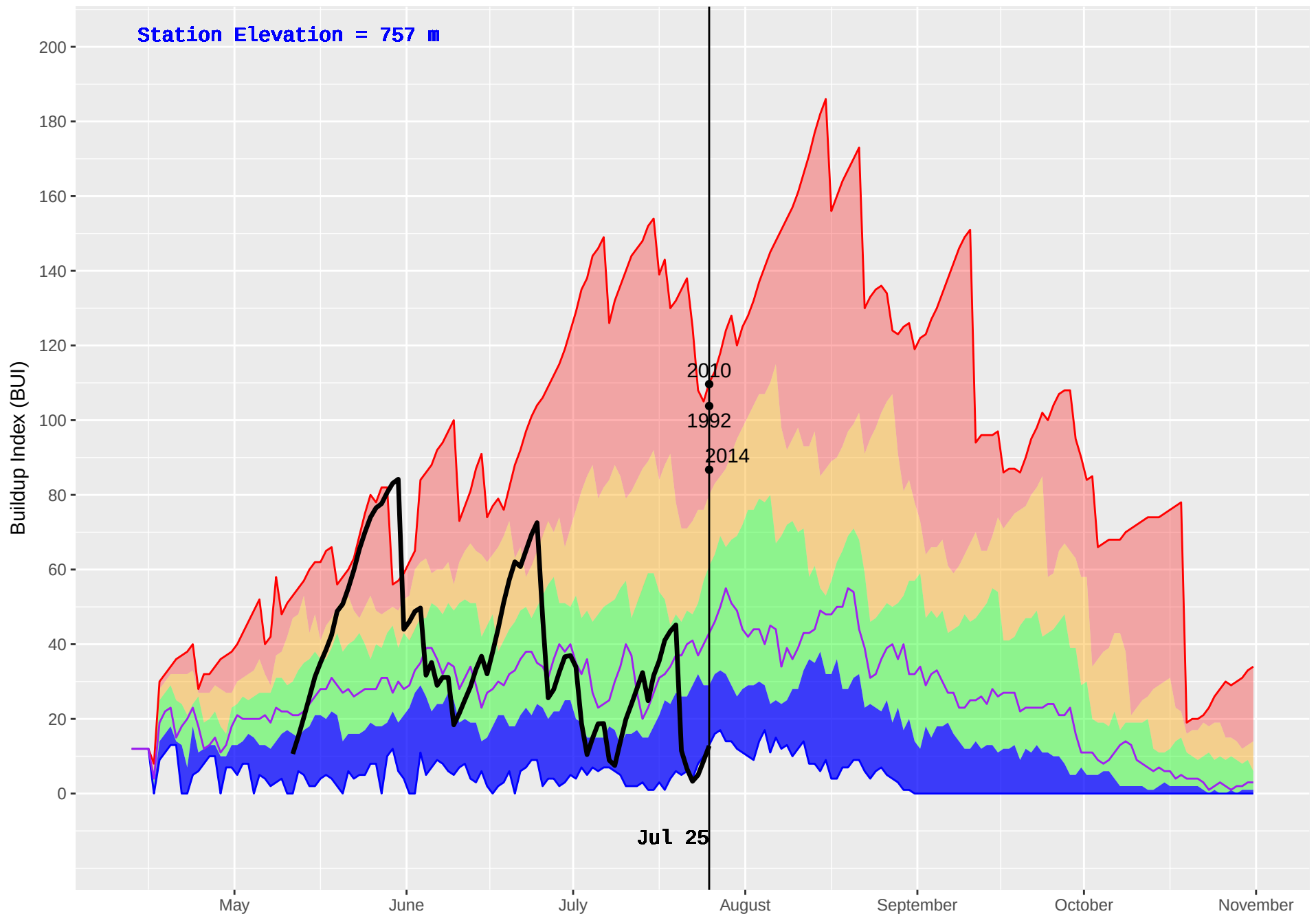
LEMORAY (140) : Historical (1988–2016) and Current (2018) Noon Buildup Index (BUI)
