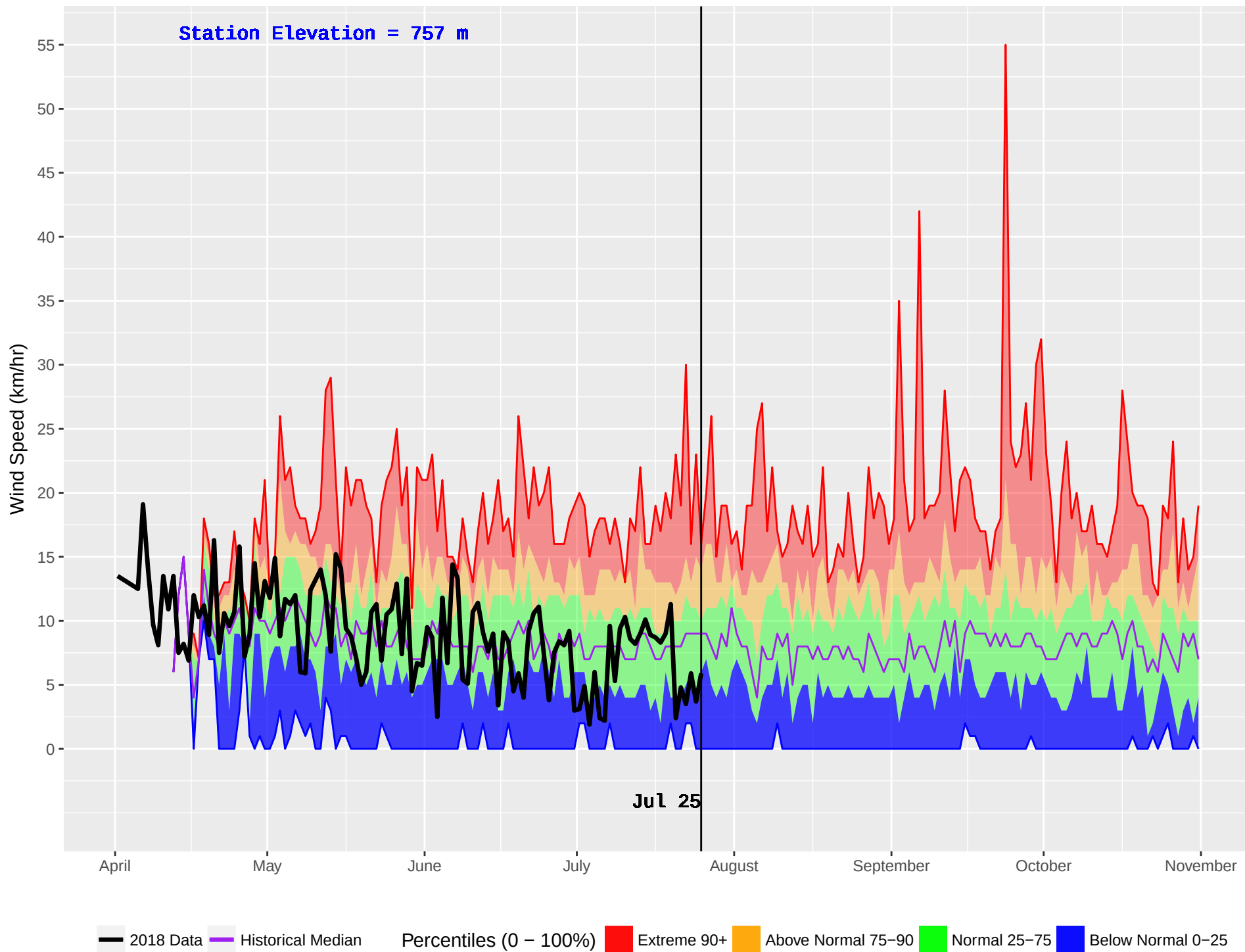
LEMORAY (140) : Historical (1988–2016) and Current (2018) Noon Wind Speed
